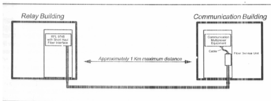
Figure 5 Typical DPLC-45 Short Haul Fiber Interface Application direct to multiplexer with C37.94 compliant I/O
